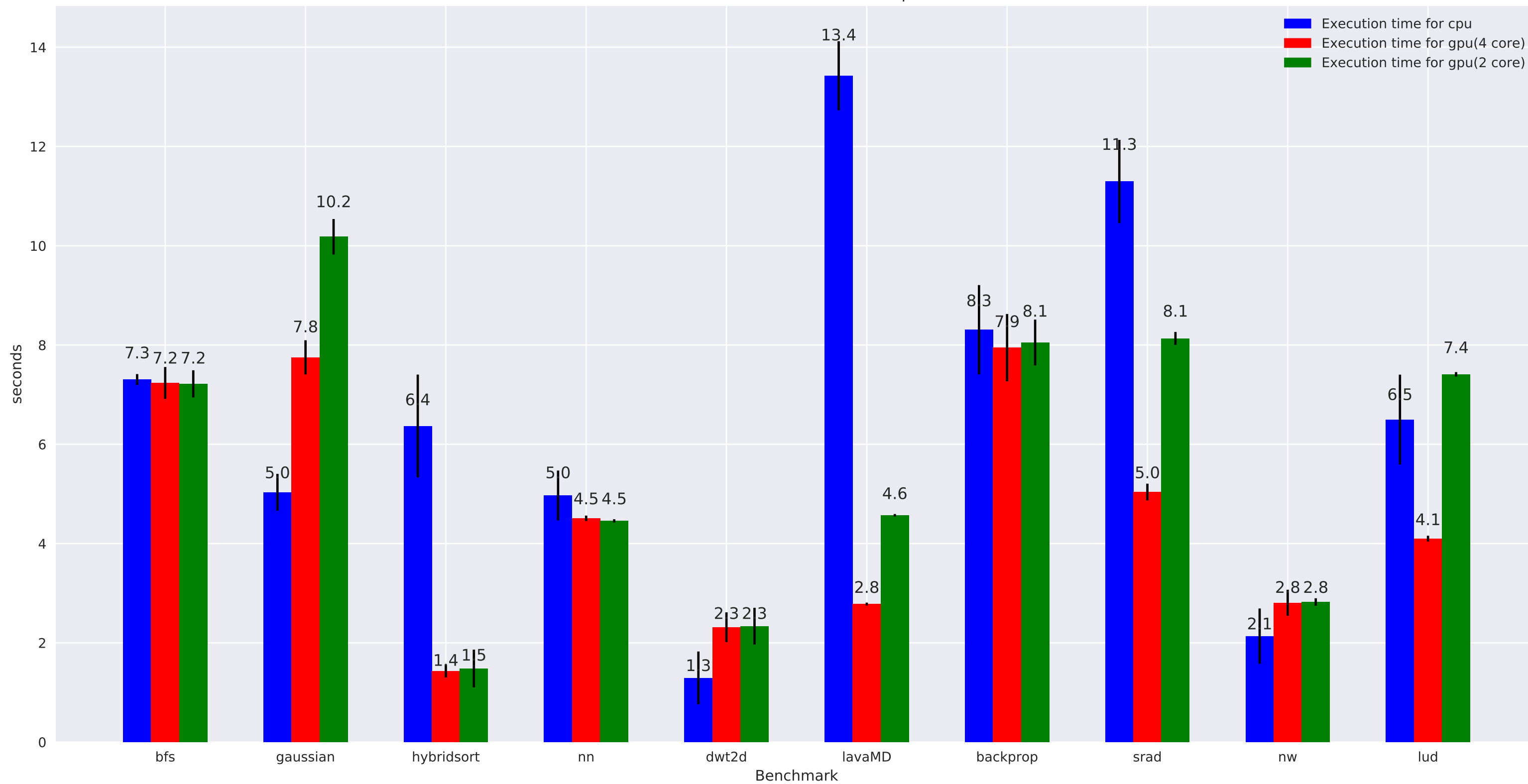
Execution time of the various benchmarks expressed in seconds
