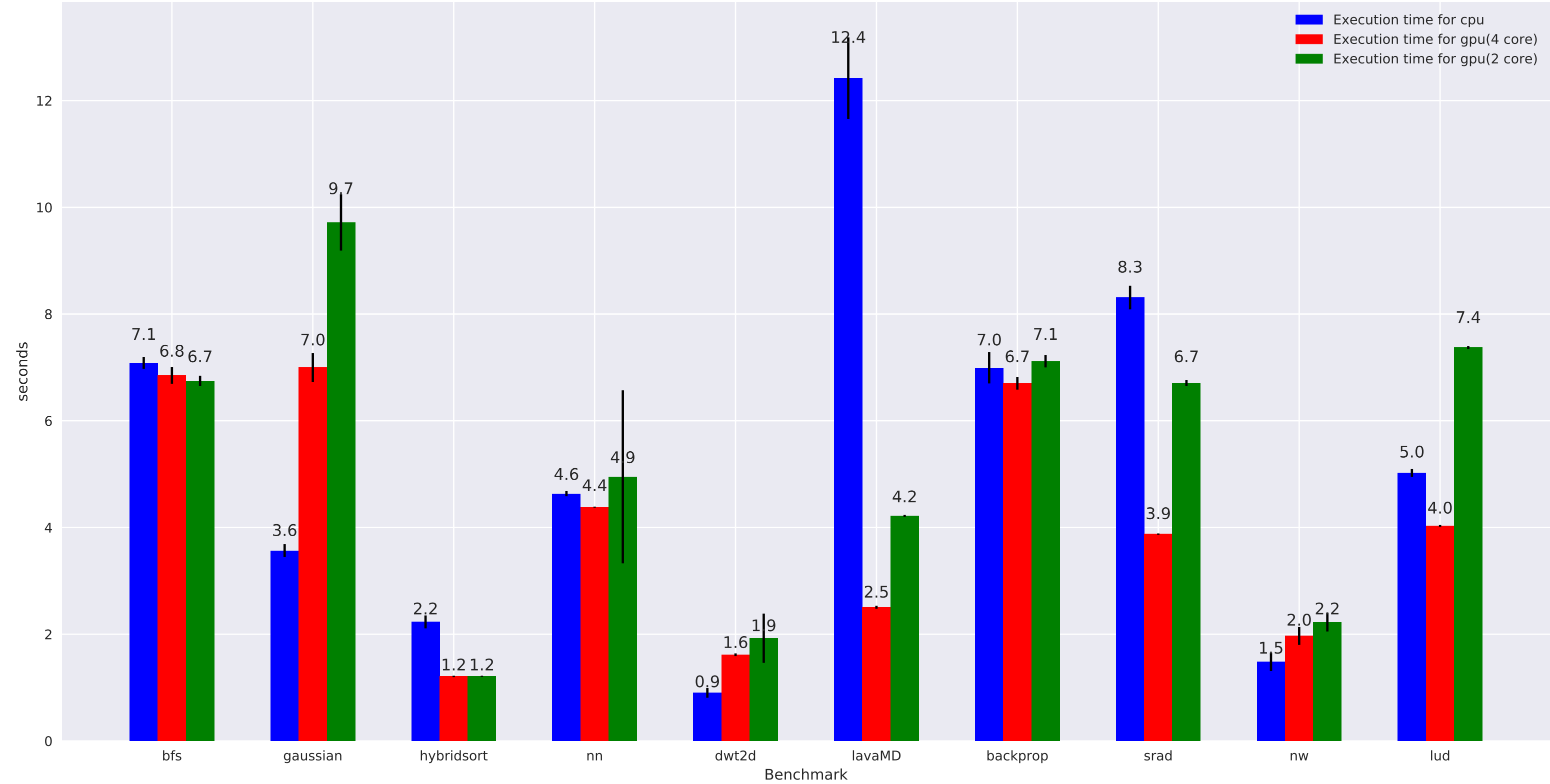
Execution time of the various benchmarks expressed in seconds
