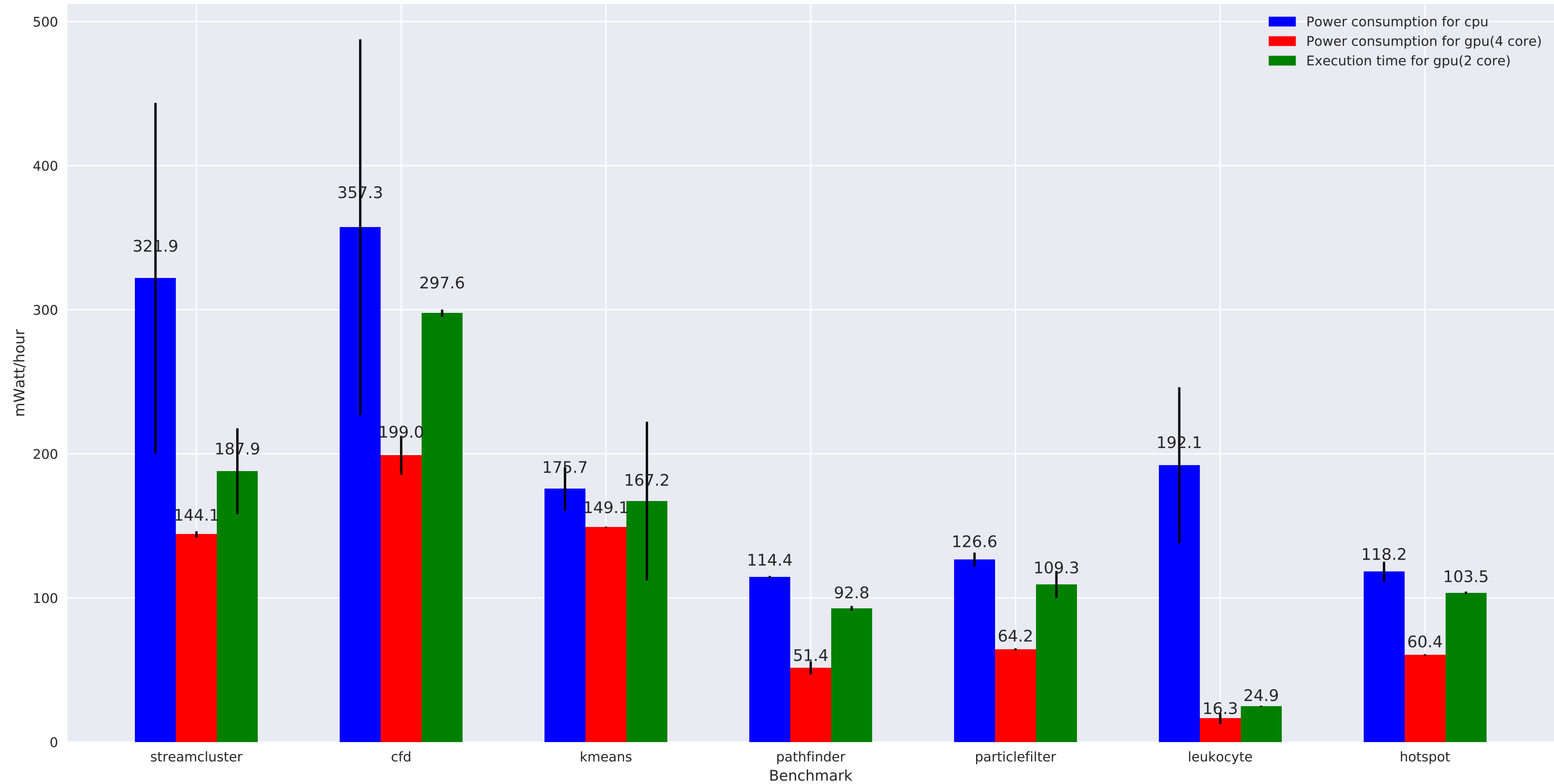
Power consumption of the various benchmarks expressed in mWatt/hour
